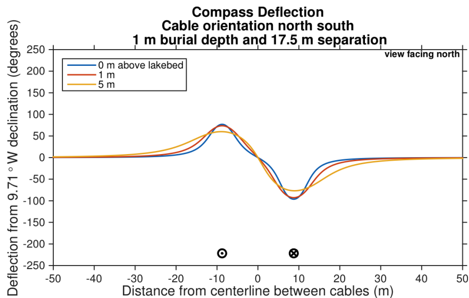
Figure A-4. Case 1. Calculated compass deflection (degrees) from 9.71^{\circ}\text{W} declination above cables oriented north-south, separated by 17.5 m in the horizontal direction and with northward current in the eastern cable.
