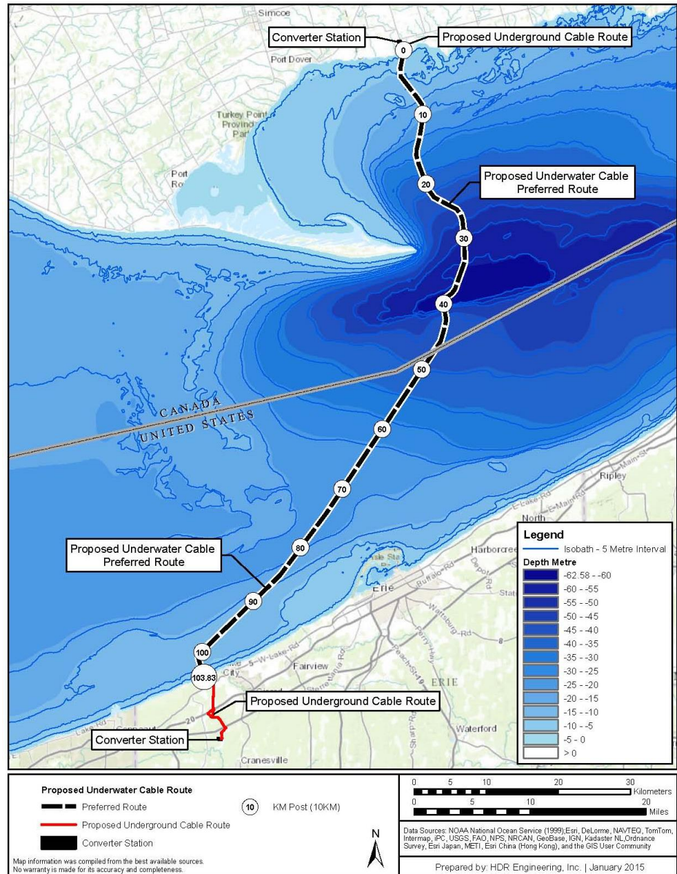
Figure 1. Proposed transmission line route across Lake Erie.
