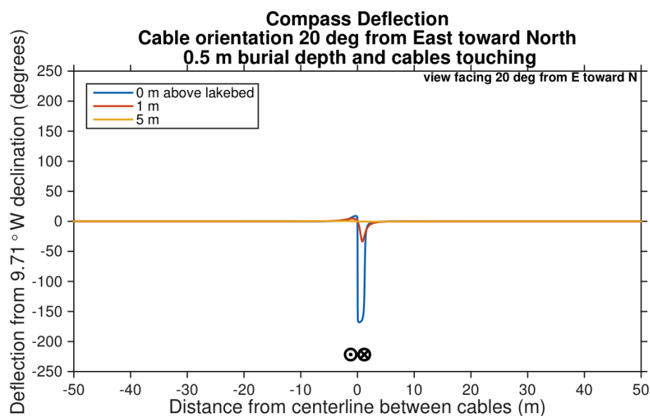
Figure A5. Case 2. Calculated compass deflection (degrees) from 9.71^{\circ}\text{W} declination above cables directed 20^{\circ} north of east, touching in the horizontal direction, and with eastward current in the southern cable.
