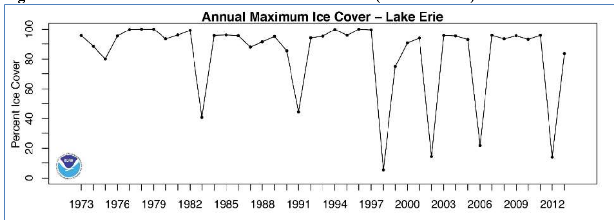
Figure 4.3-1 Annual maximum ice cover in Lake Erie (NOAA 2014a).
