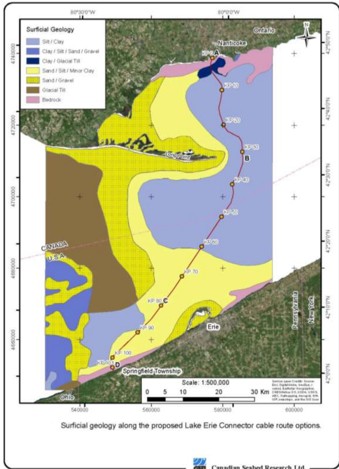
Figure 4.2-1 Generalized geological map of the of the proposed transmission line route in Lake Erie.
