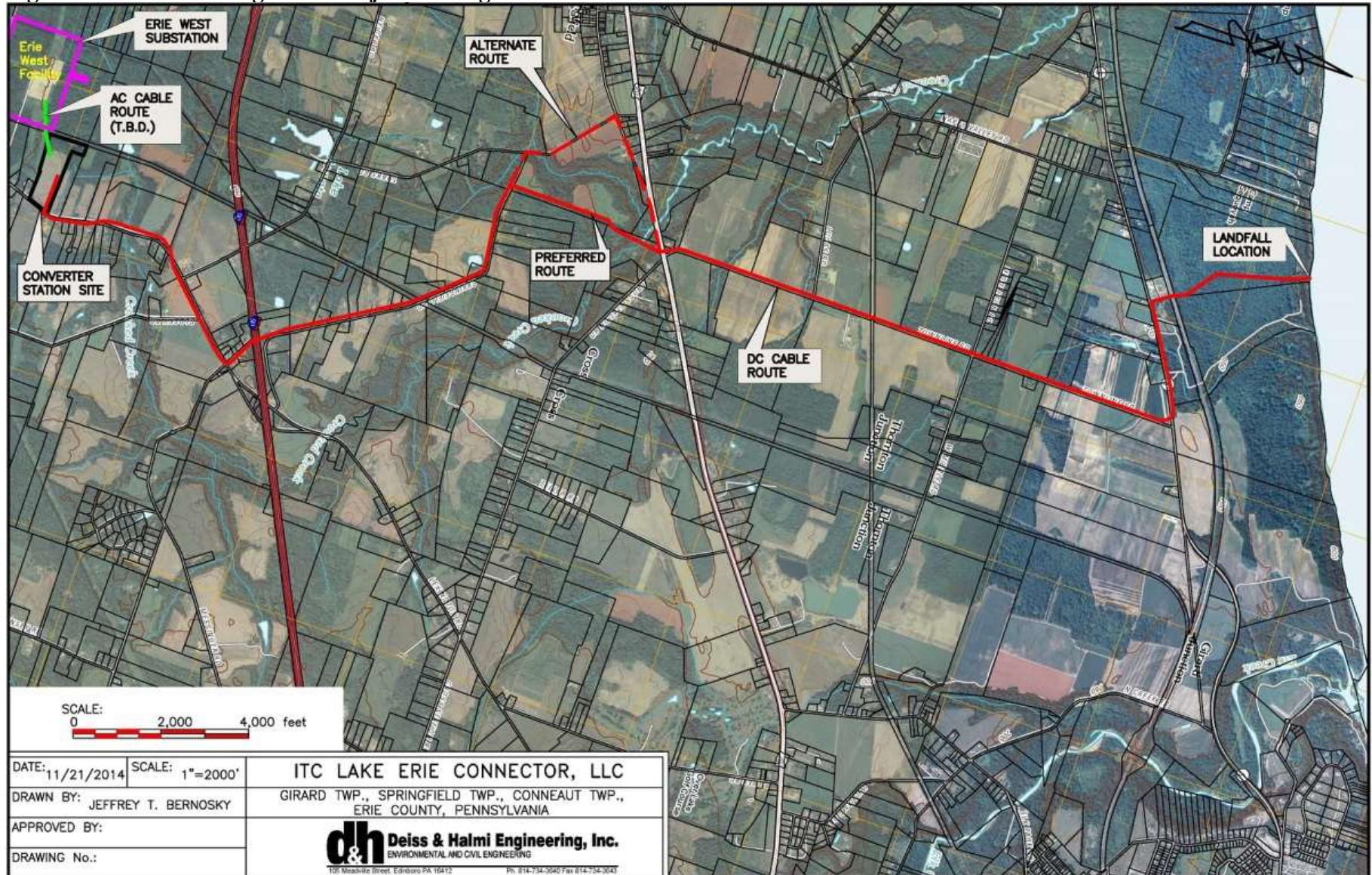
Figure 2.2-3 Underground Project routing.
