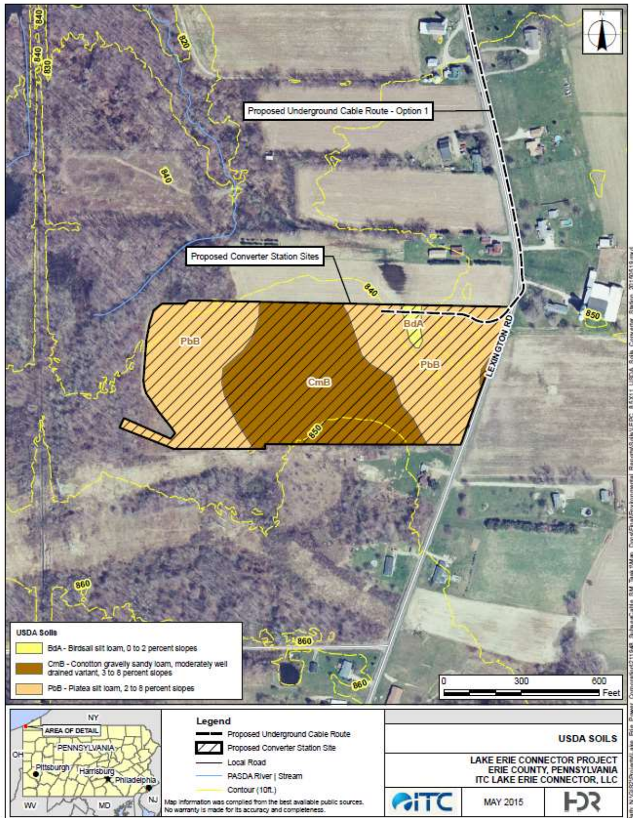
Figure 4.2-3 Converter station site soil survey.
