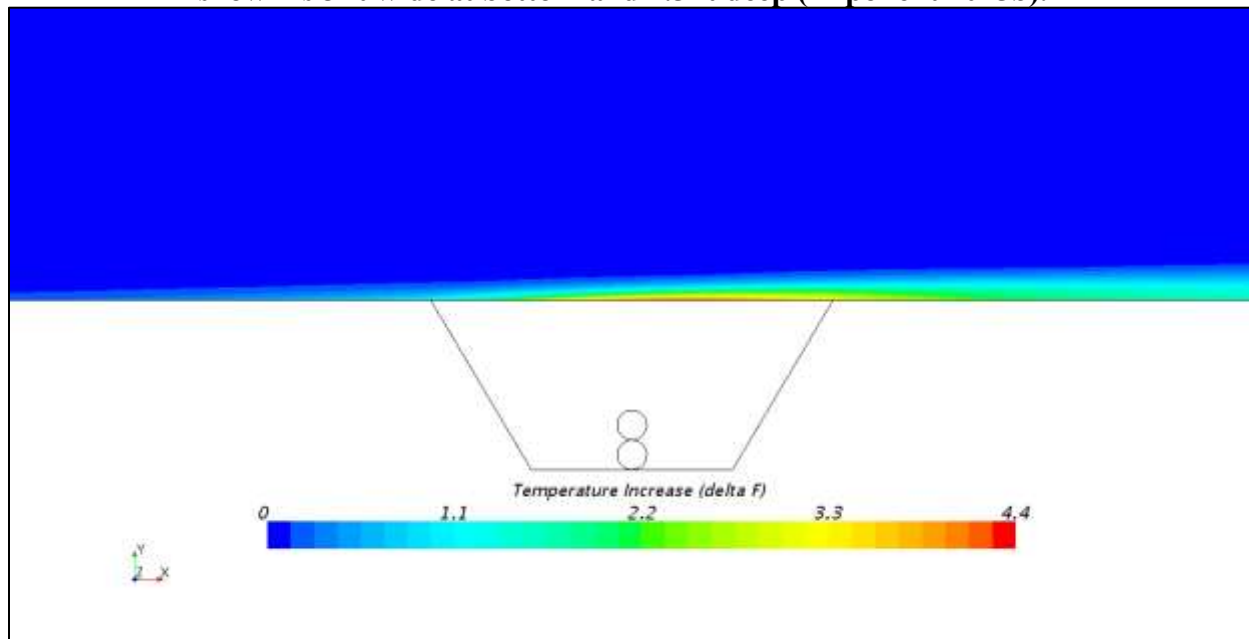
Figure 5.3-1 Calculated thermal effects of Project transmission line: bedrock trench shown is 3 ft wide at bottom and 2.5 ft deep (Exponent 2015b).
