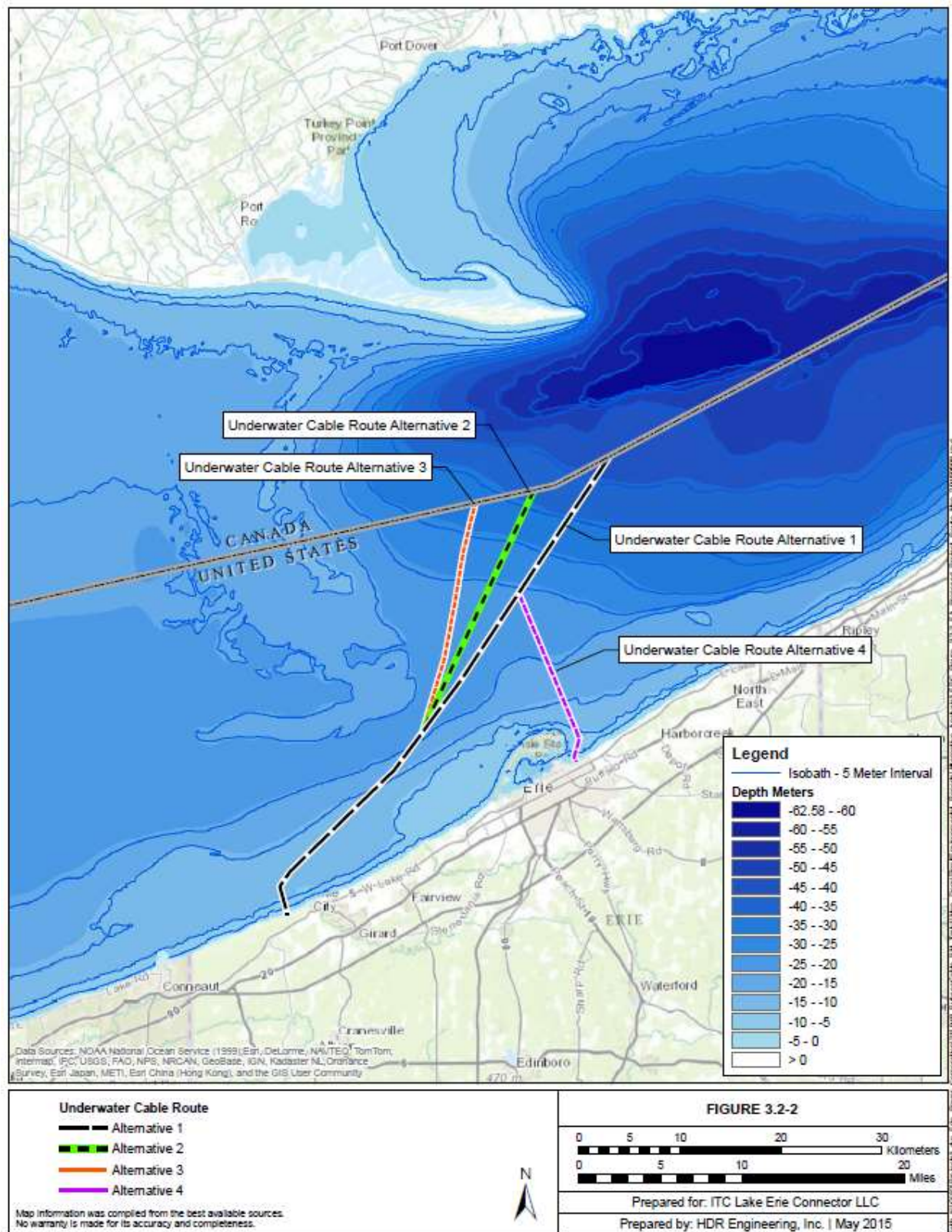
Figure 3.2-2 U.S. underwater alternatives.
