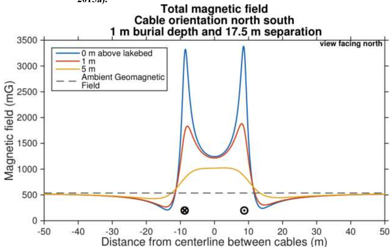
Figure 5.4-3 Calculated magnetic field profile for cables oriented north-south and buried at a depth of 1 m. The cables are separated by 17.5 m (Exponent 2015a).
