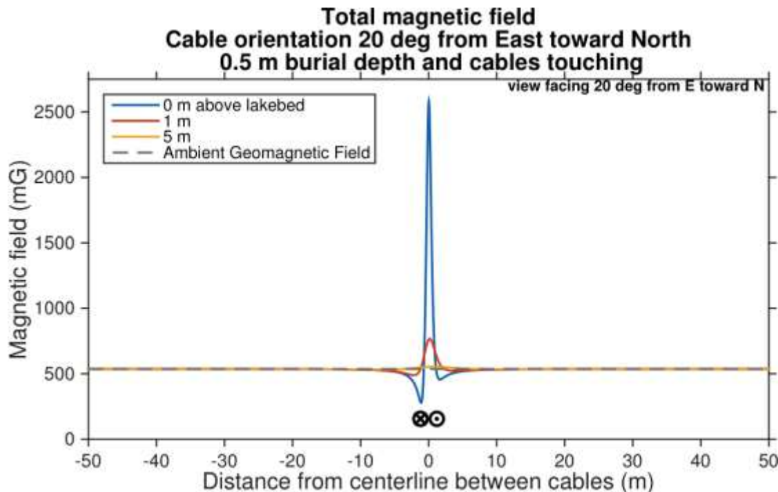
Figure 5.4-2 Calculated magnetic field profile for cables strapped together, laid horizontally and oriented at 20° north of east and buried at a depth of 0.5 m (Exponent 2015a).
